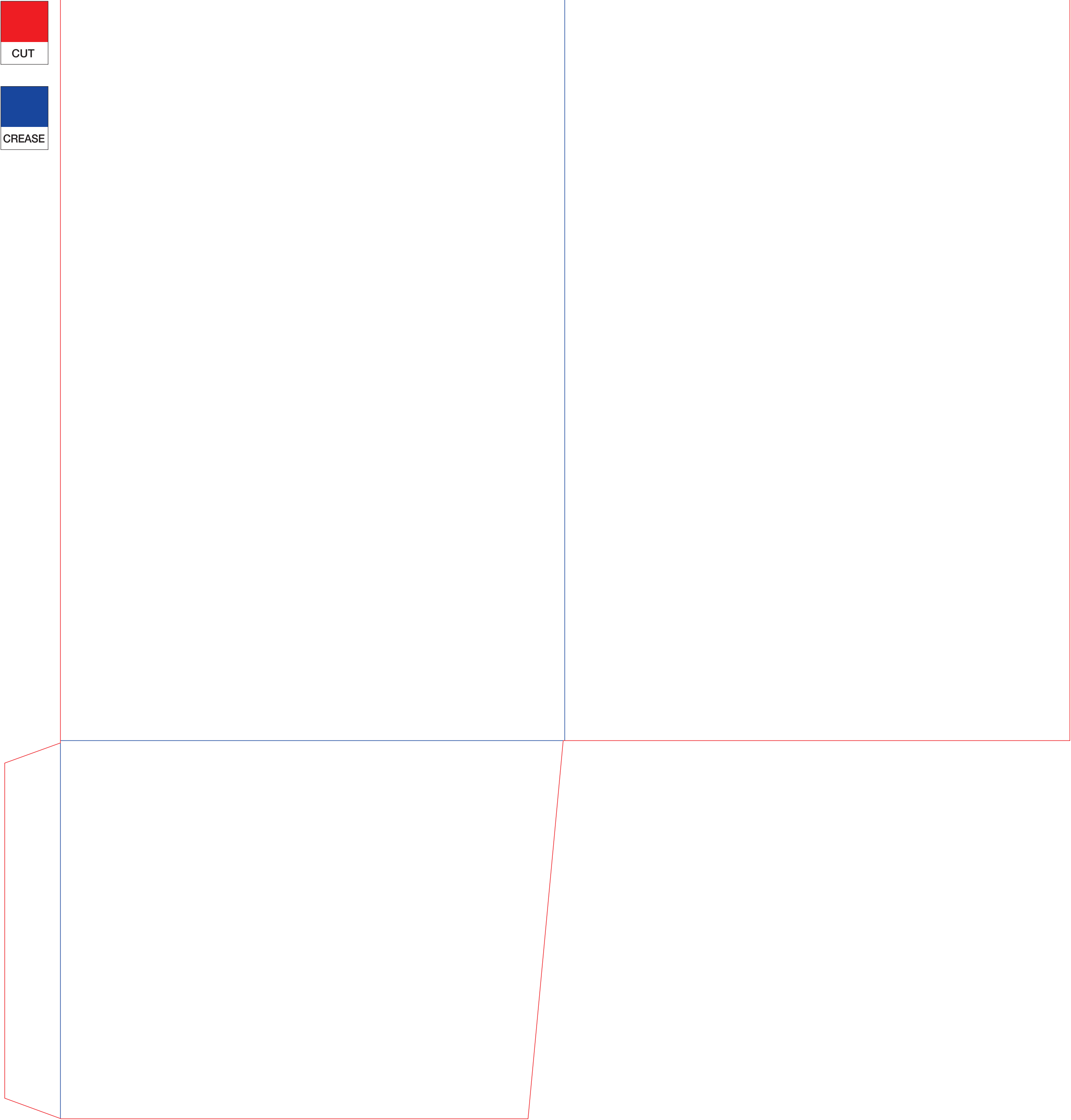
Die Line: One-Piece 6" x 9" Single Pocket Folder - No Gusset
